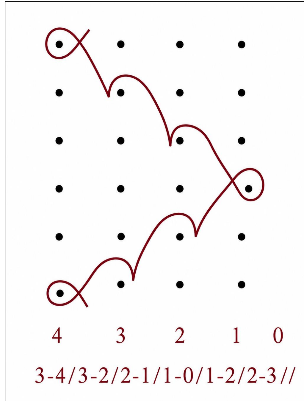
Three Course Tricot Atlas
